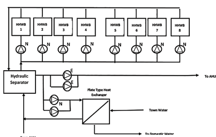
Proposed Heating Hot Water Boiler (HHWB) System
